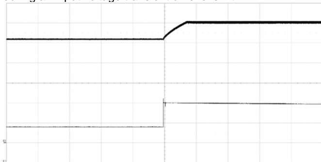
HRR product output at input voltage step 36-60 V, 10 ms/div Bottom trace – input voltage change 36-60 V, 20 V/div Top trace – resulting output voltage change, 2 V/div
