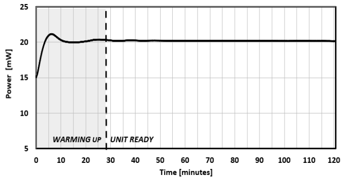
FIG. 9: WARM-UP TIME
