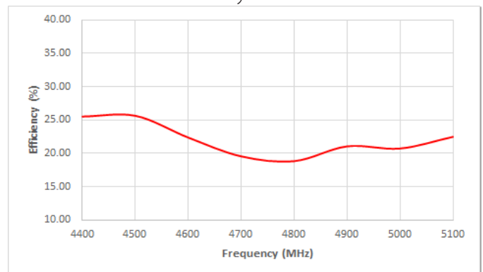
Efficiency - C-Band
