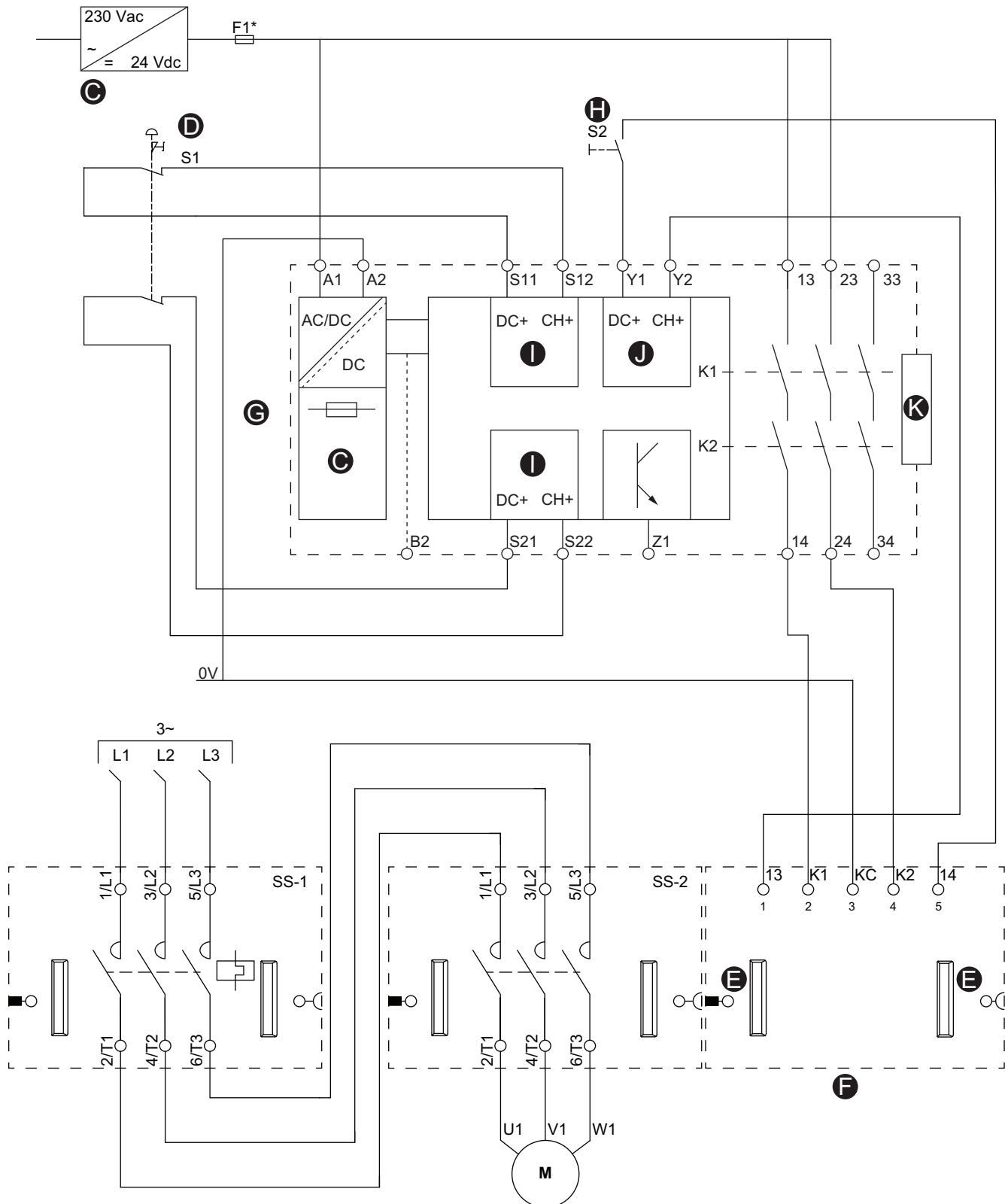
Figure 22 - Example: SIL Stop, Stop Category 0, Wiring Category 3/4 32
