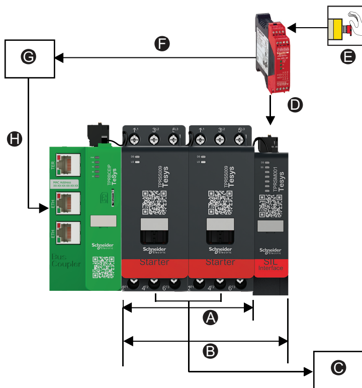
Figure 10 - Stop Command
