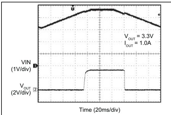
FIGURE 2-45: UVLO Thresholds.
