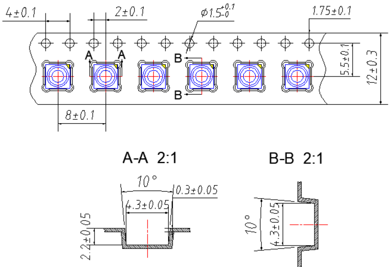
Figure 9: Carrier Tape (1)
