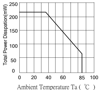
Ambient Temperature vs. Total Power Dissipation
