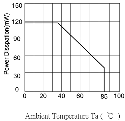
Ambient Temperature vs. Total Power Dissipation
