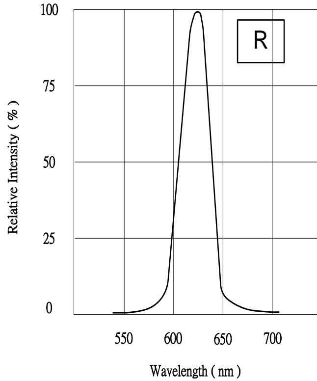
Relative Intensity vs Wavelength
