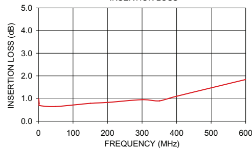
TC4-6TG2+ INSERTION LOSS
