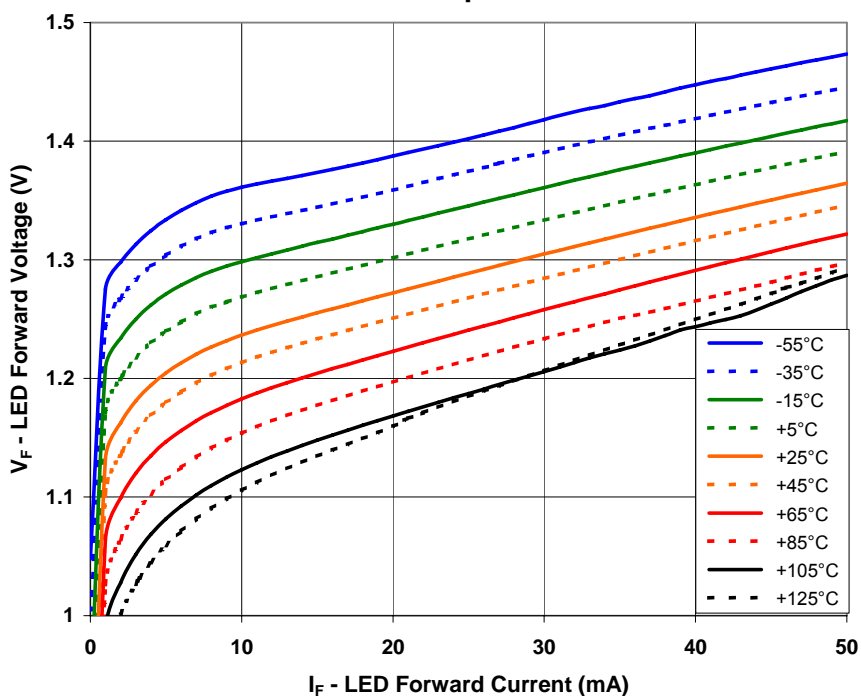
Forward Voltage Vs Forward Current Vs Ambient Temperature
