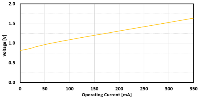
FIG. 13: SLED 2 FORWARD VOLTAGE VS CURRENT
