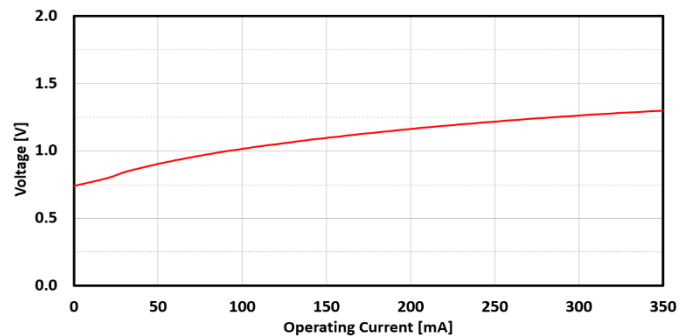
FIG. 14: SLED 3 FORWARD VOLTAGE VS CURRENT
