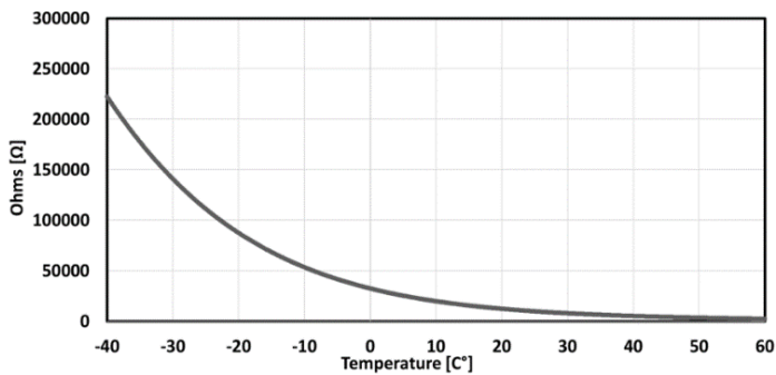
FIG. 17: THERMISTOR R_{THTEC} RESISTANCE VS TEMPERATURE
