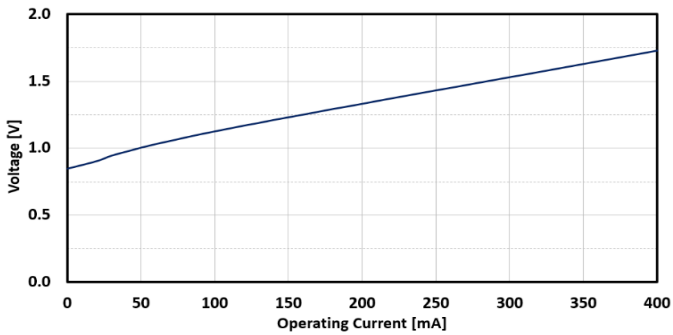
FIG. 15: SLED 4 FORWARD VOLTAGE VS CURRENT
