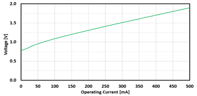
FIG. 12: SLED 1 FORWARD VOLTAGE VS CURRENT
