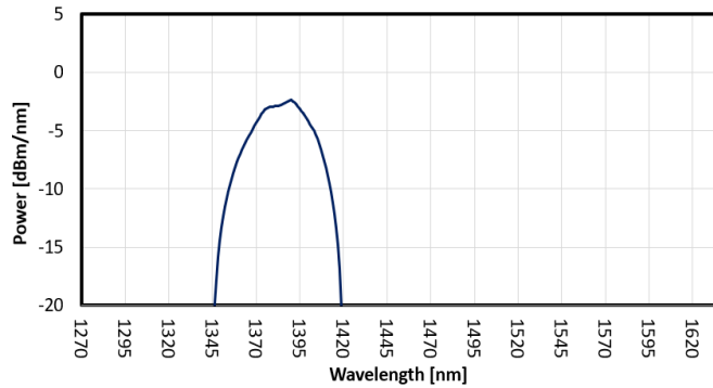
FIG. 5: SLED 4 SPECTRUM
