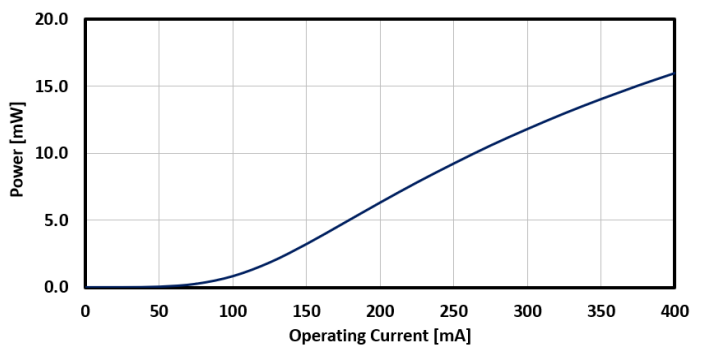
FIG. 10: SLED 4 OUTPUT POWER VS CURRENT
