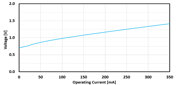
FIG. 16: SLED 5 FORWARD VOLTAGE VS CURRENT
