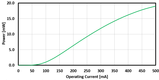
FIG. 9: SLED 3 OUTPUT POWER VS CURRENT
