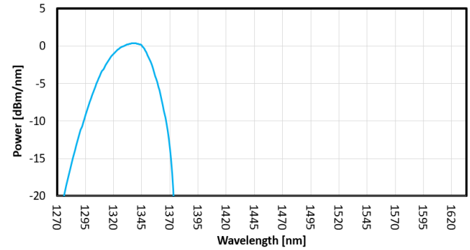
FIG. 6: SLED 5 SPECTRUM
