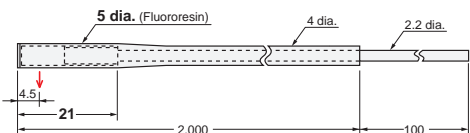
39-E E32-T51F 2M (Free Cutting)
