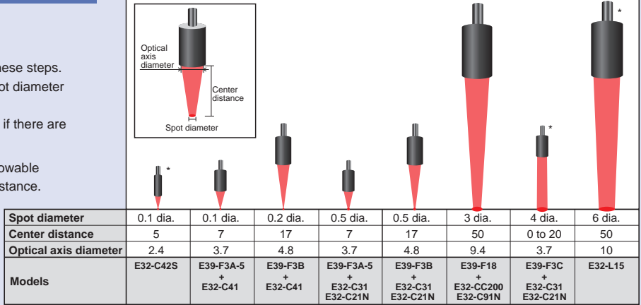
<Map of Spot Diameters and Center Distances> (Unit: mm)
