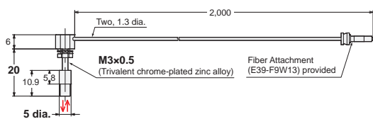
21-D E32-C21N 2M (Free Cutting) + E39-F3C
