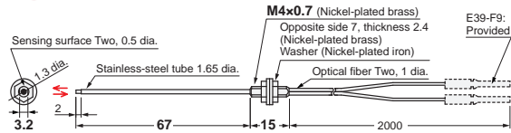
19-J E32-D21-S3 2M (Free Cutting)
