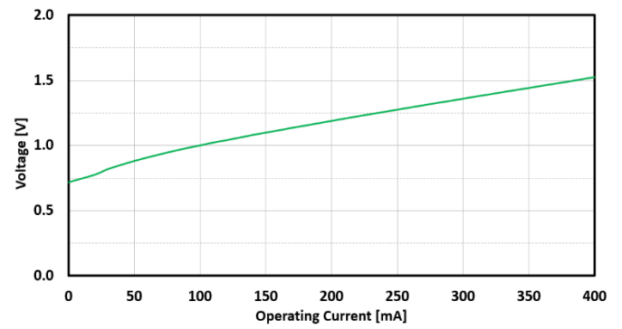
FIG. 14: SLED 1 FORWARD VOLTAGE VS CURRENT
